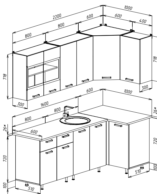
РИО NEW 2,2x1,0 (490)
